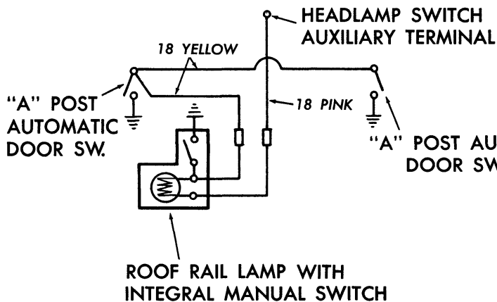
Wiring Diagram—Interior Lighting
