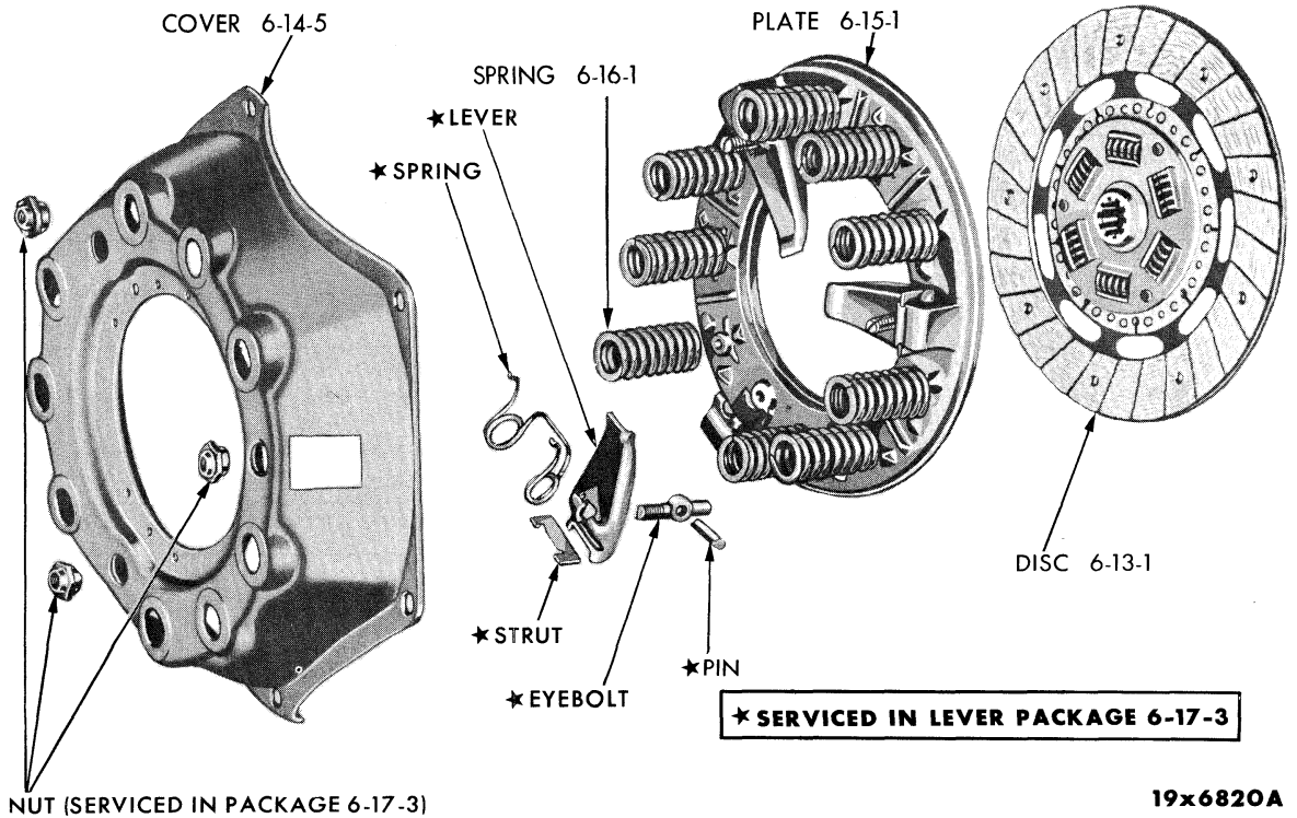
CLUTCH - TYPE 2
