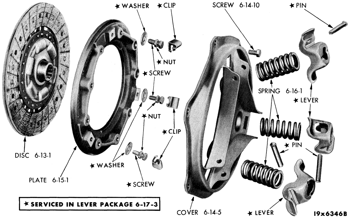
CLUTCH - TYPE 1
