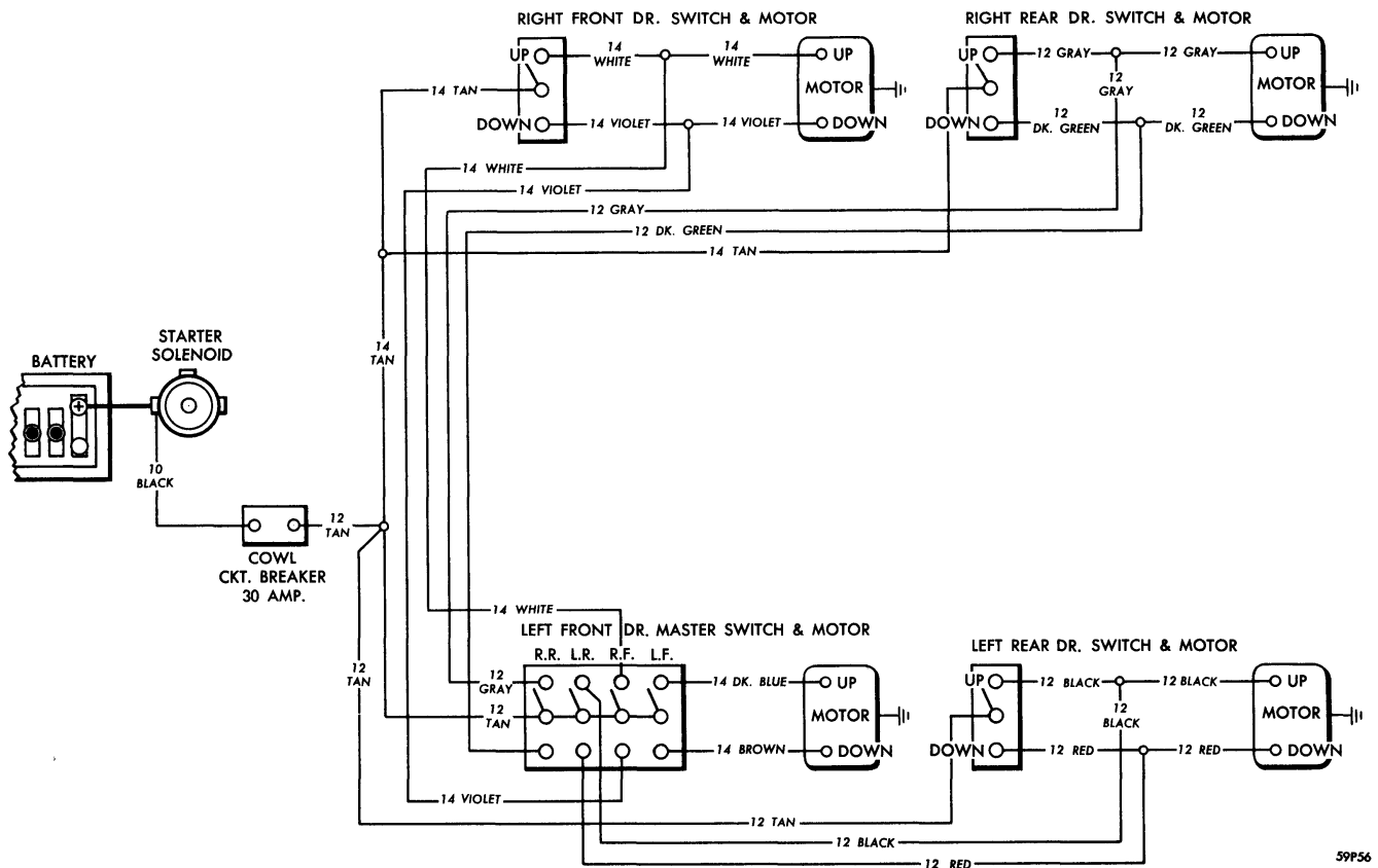
Wiring Diagram—Electric Window Lift
