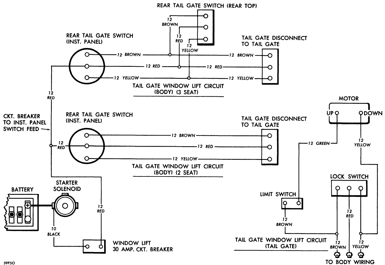
Wiring Diagram—Tailgate Window Lift
